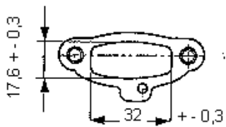
CYLINDER INTAKE FLANGE
