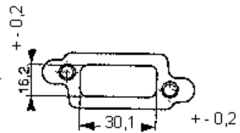
CYLINDER EXHAUST FLANGE
